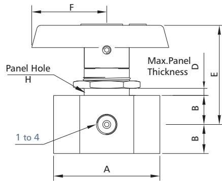
4-way Valves
