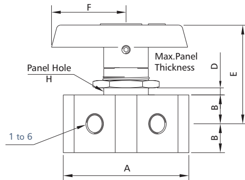
6-way Valves
