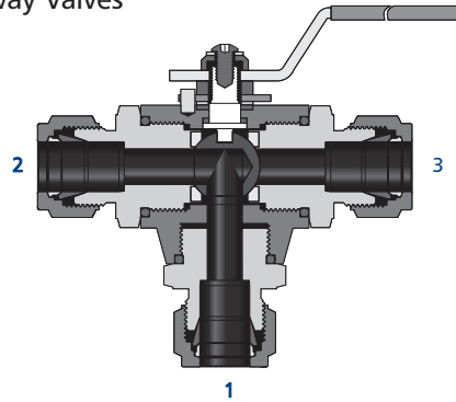
3-way Valves
