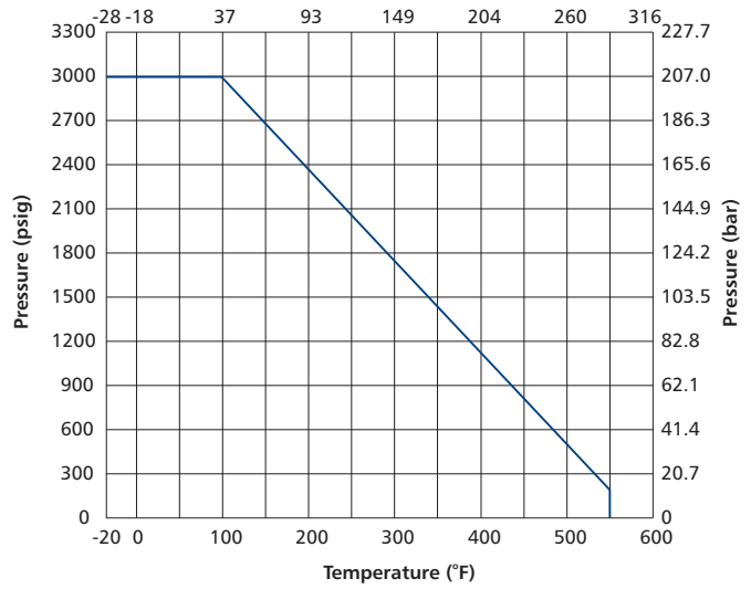
PEEK Seat Temperature (°C)
