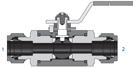
2-way Valves
