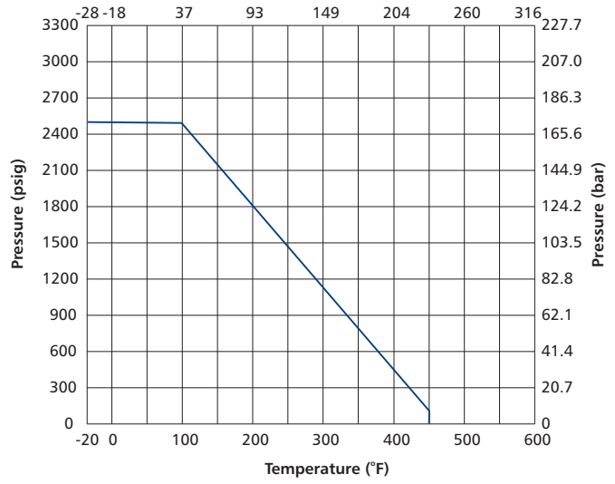
Reinforced PTFE Seat Temperature (°C)
